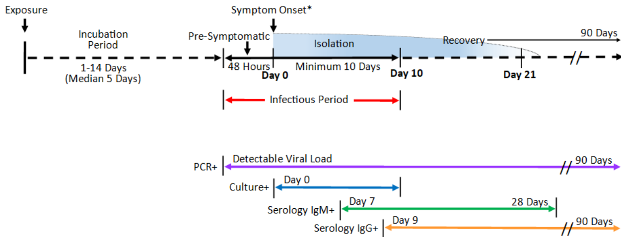
FIGURE 5.1 INCUBATION, INFECTIOUS PERIOD, AND TEST POSITIVITY FOR SARS-COV-2
